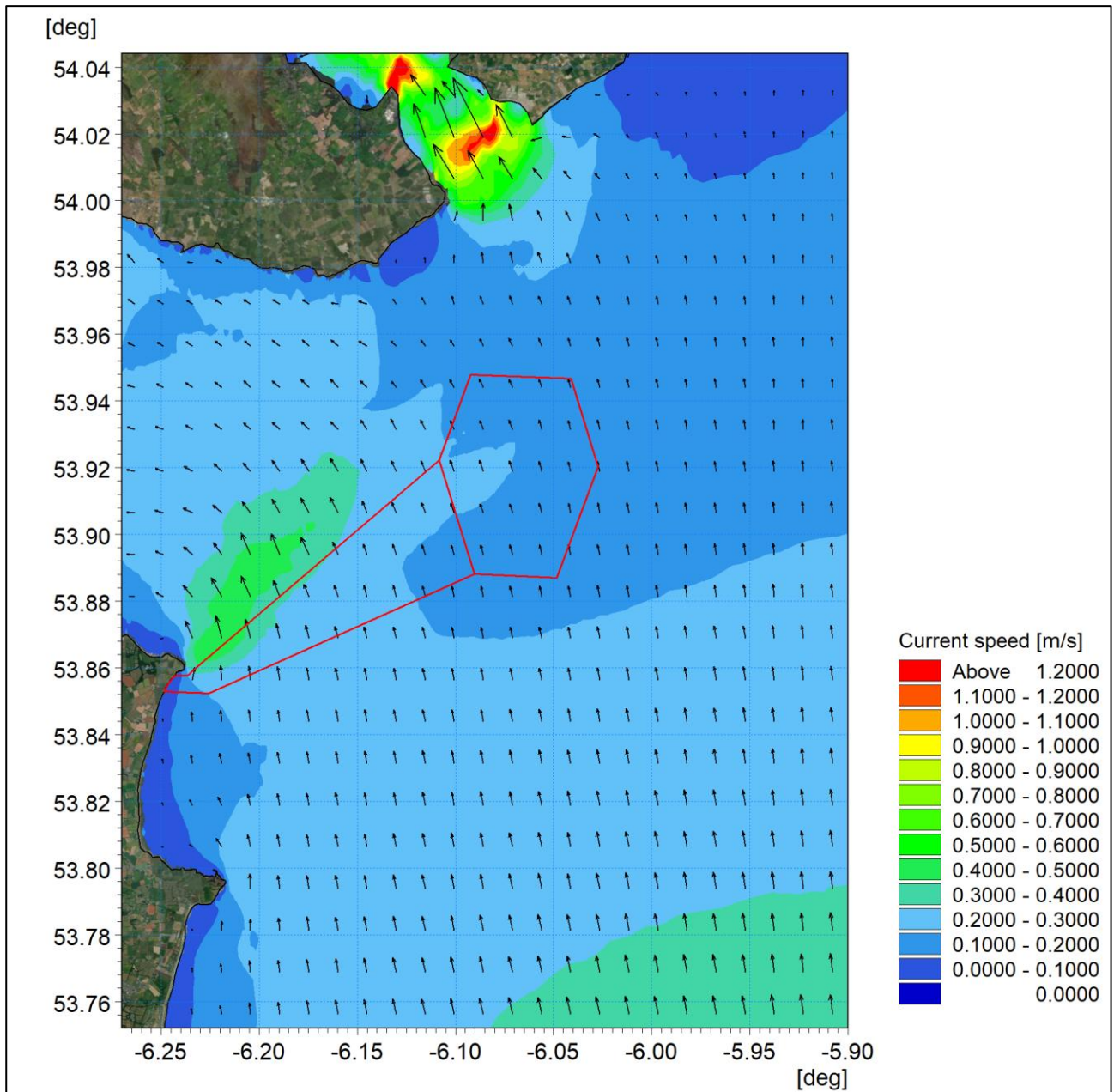
Figure 3-3: Post-construction tidal flow patterns - mid-flood.
