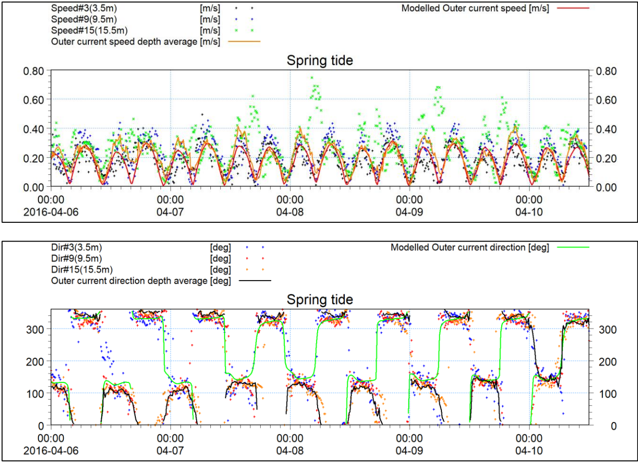
Figure 4A-9: Measured and modelled Outer current speed (upper) and direction (lower) – spring tide.
